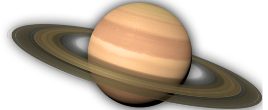
Saturn
