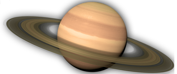
Saturn
