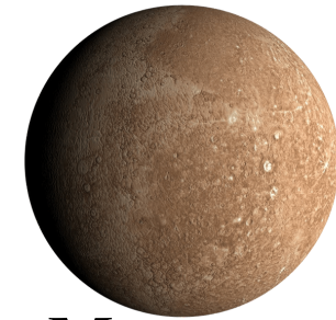
Mercury
