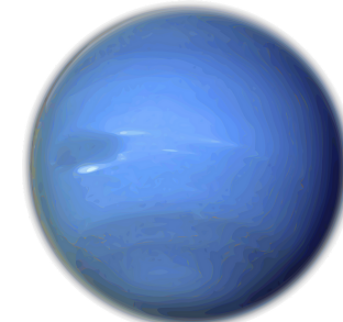
Neptune
