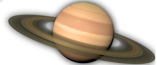
Saturn
