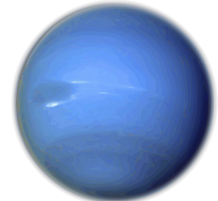
Neptune
