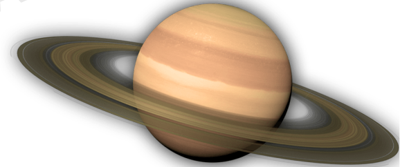
Saturn
